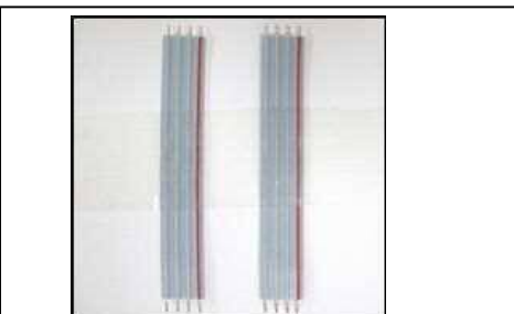
P / N : QUM024-07A2Z3 ( UL2651-26 ) application for Home Audio (DVD)
